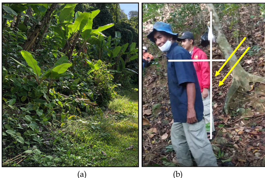
Figure 6. (a) Vegetation Condition of the Studied Area, (b) Slow Flowage in the Studied Area
