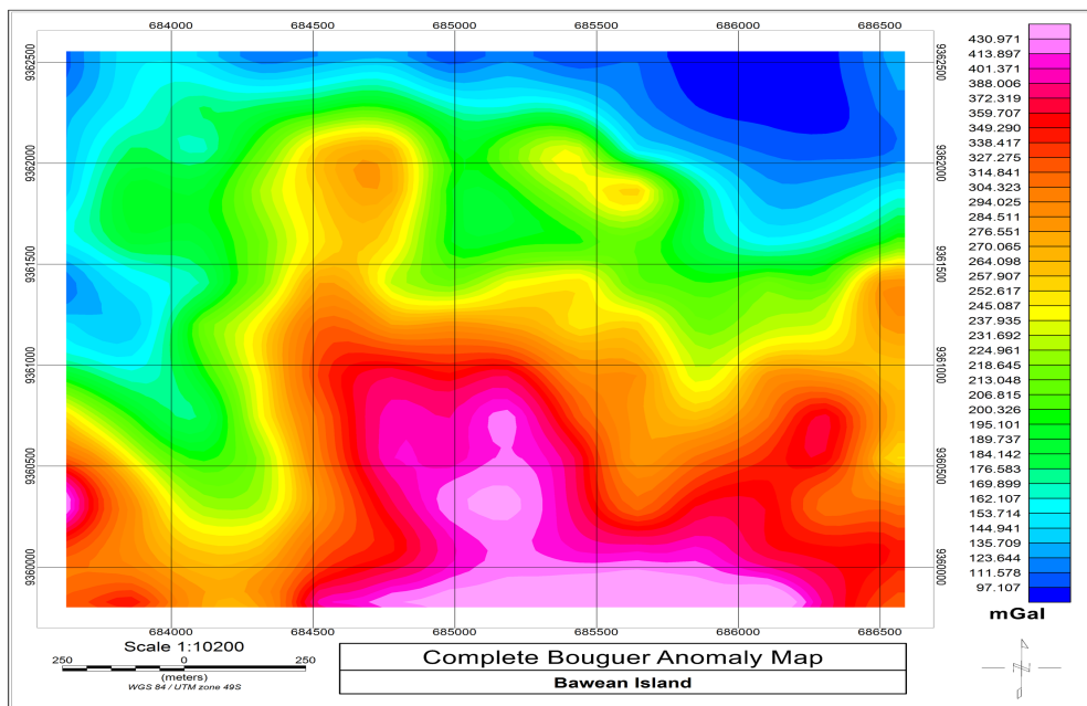
Figure 2. Complete Bouguer Anomaly Map in the Kastoba Lake Area.
