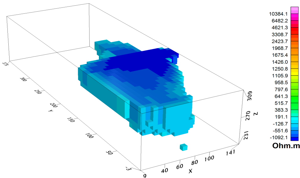
Figure 7. The Results of the 3D Interpretation of the Distribution of Low Resistivity Values.
