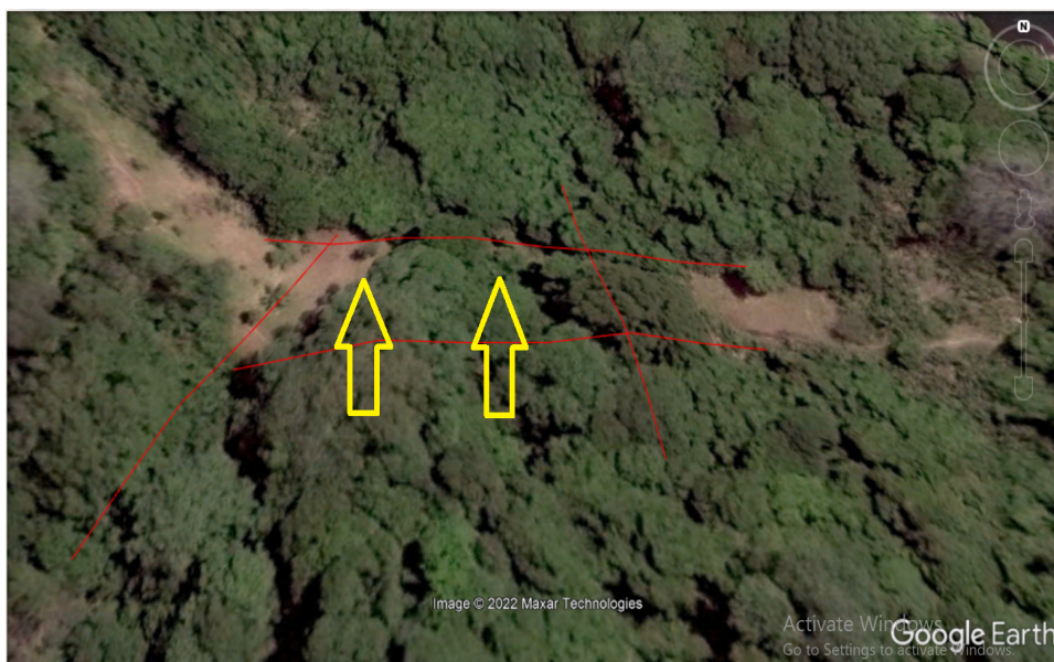
Figure 8. Landslide Direction Based on Visual Observation
