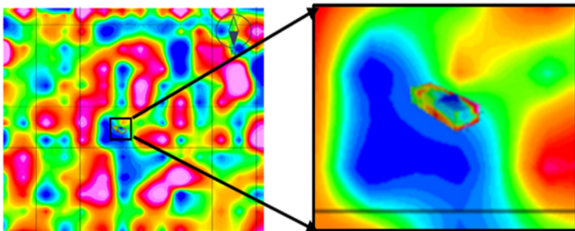
Figure 5. Correlation of Bouguer Anomaly Maps and Resistivity 3D Results.
