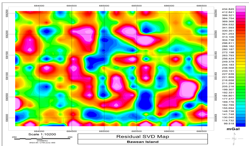
Figure 3. Residual Anomaly Map in the Geotourism Area of Kastoba Lake.
