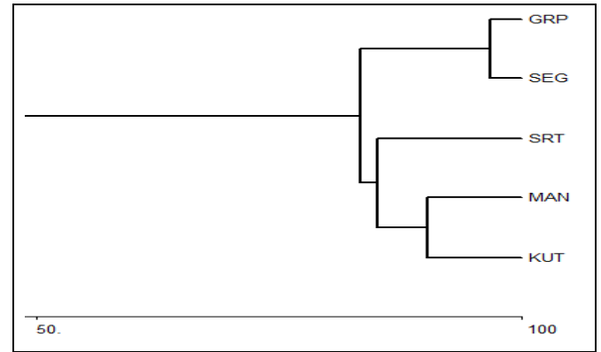
Figure 3. Percentage similarity of among sampling points
