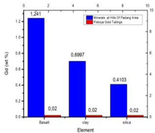
Figure 2. Gadolinium Extraction Result Diagram
