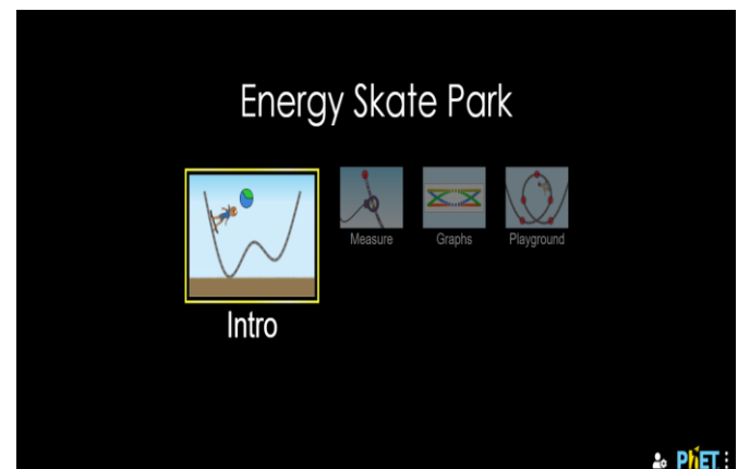
Figure 1. PhET simulations experiments on energy materials
